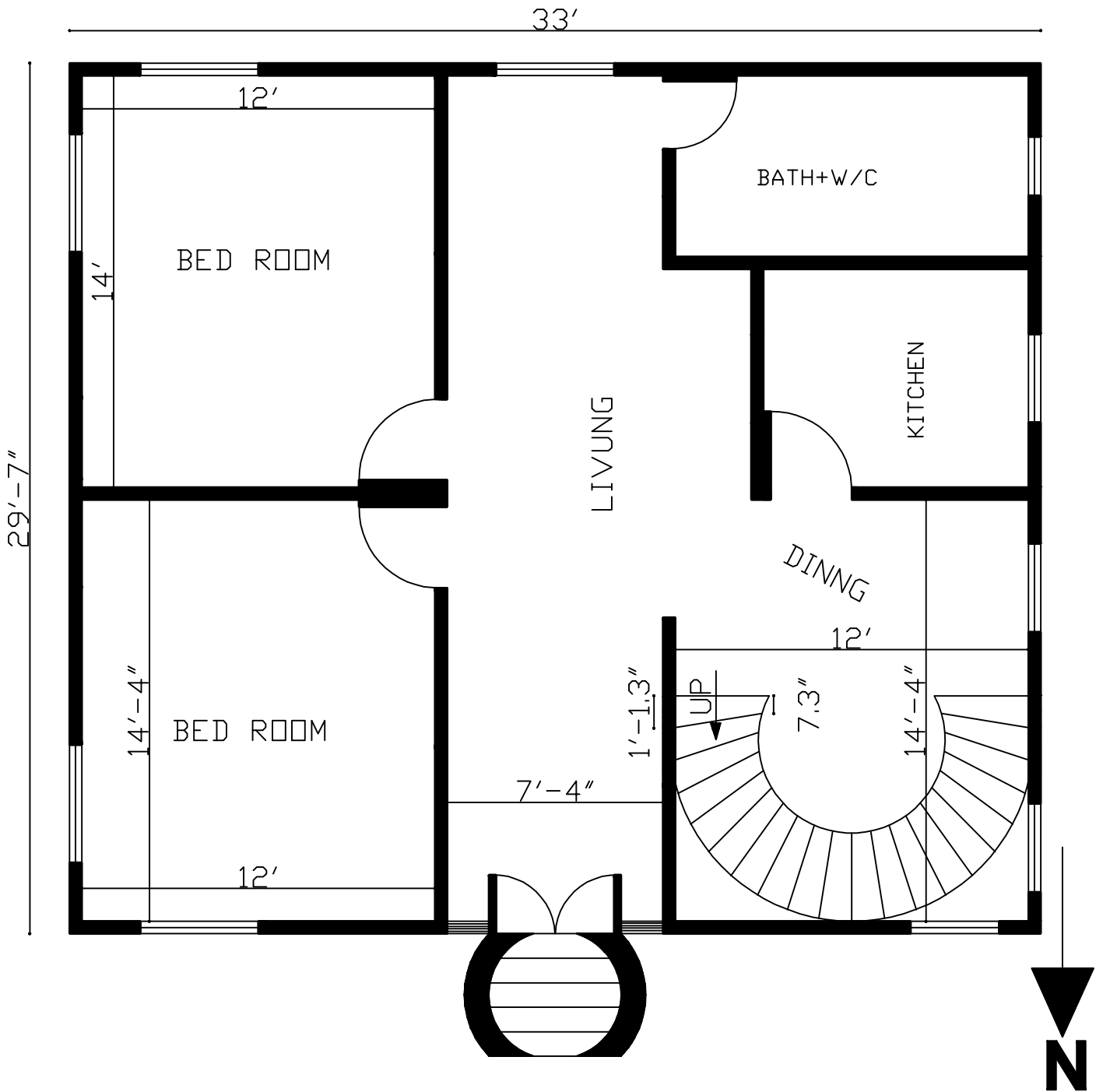
33'x29' 2 BEDROOM HOUSE
