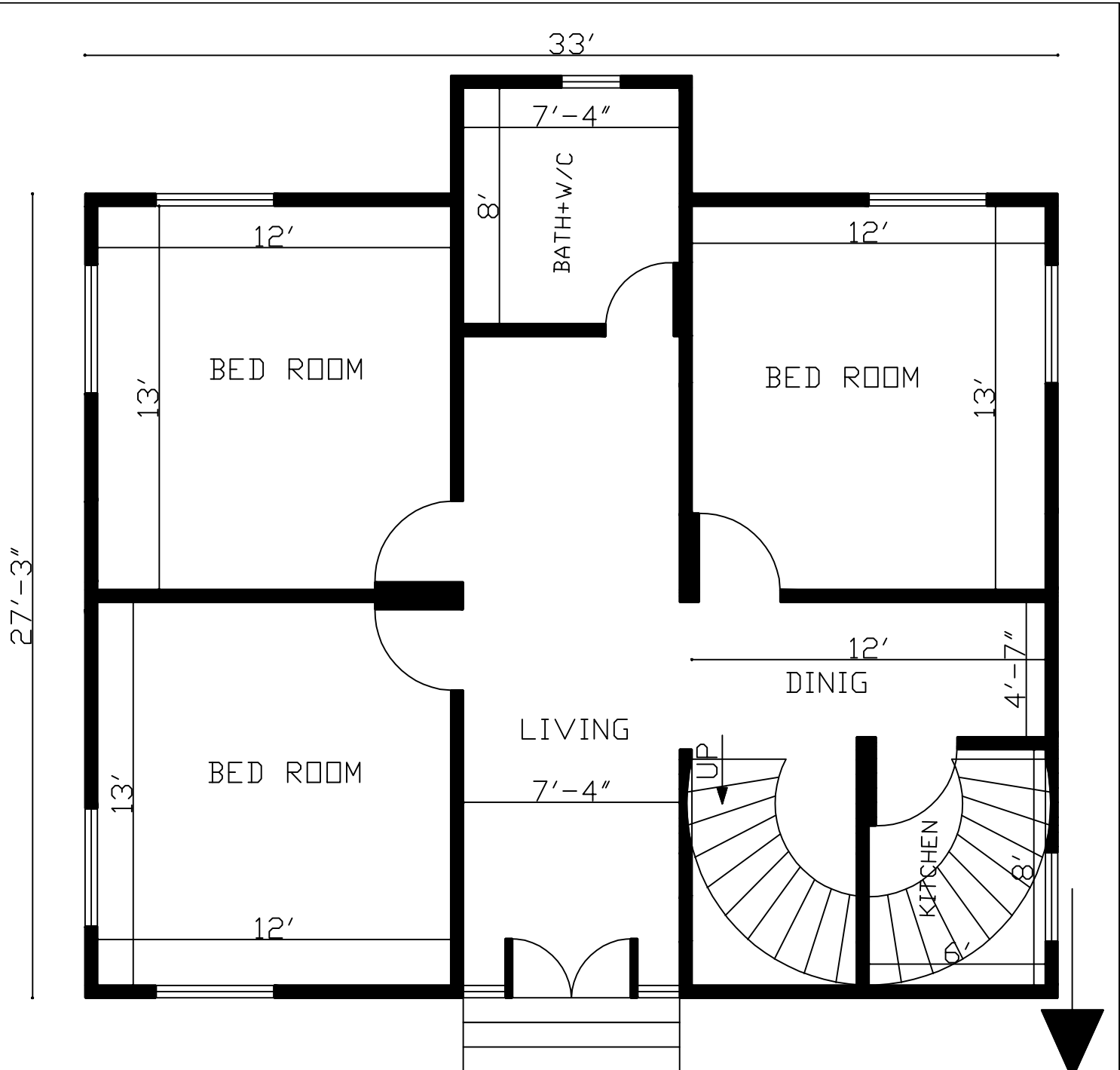
33'x27' 3 BEDROOM HOUSE
