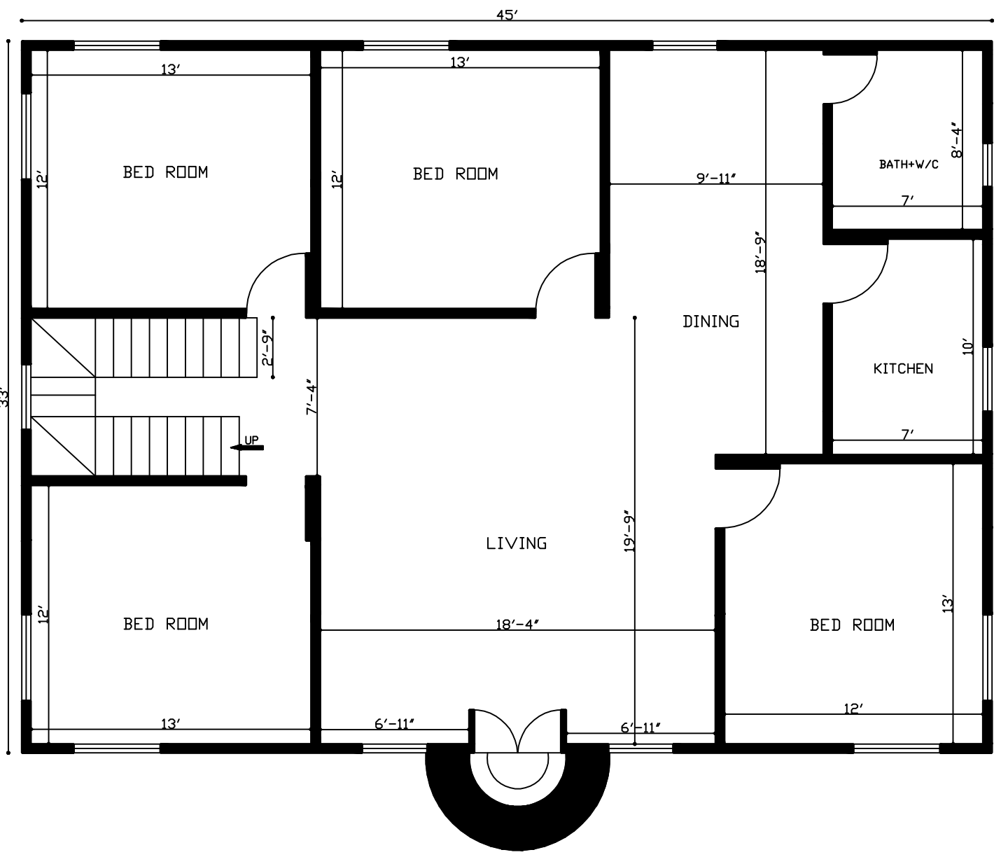
33'X45' 1500 Sq. Ft. House Plan
