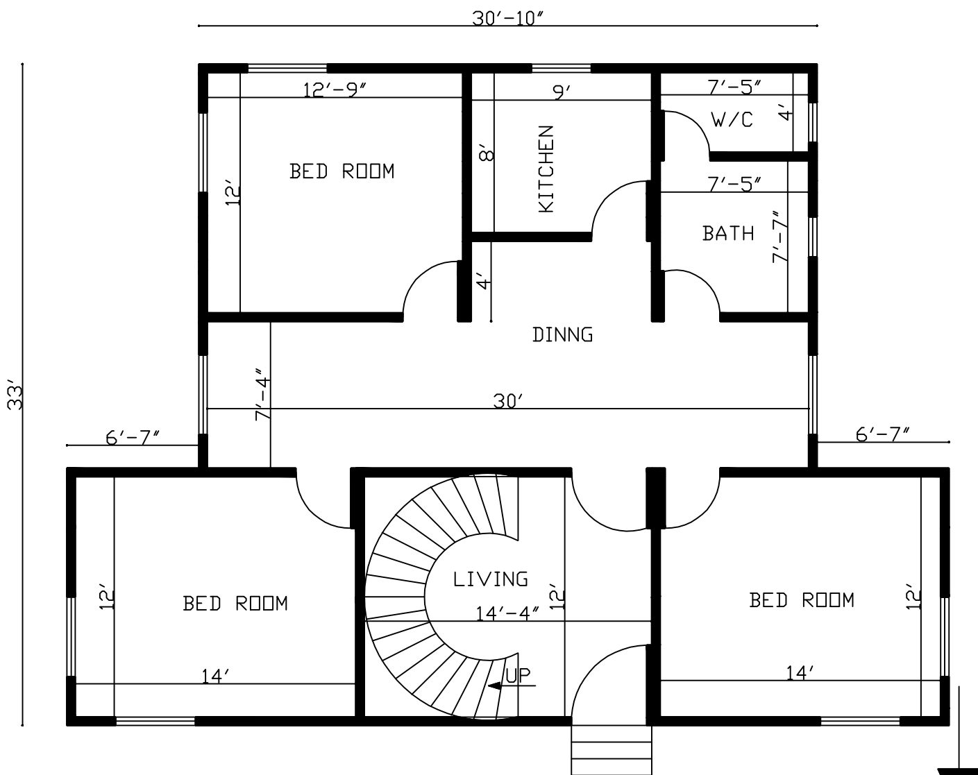
33'x31' 3 BEDROOM HOUSE
