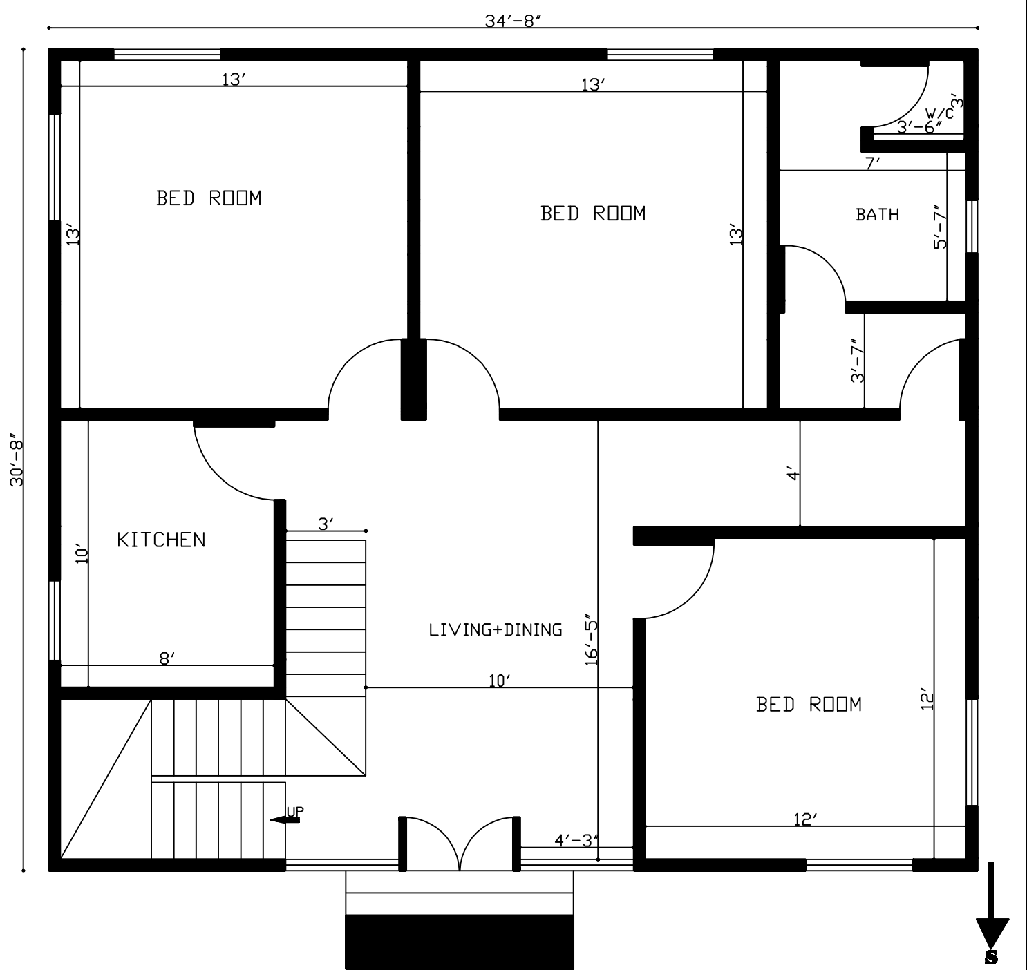
31'X35' 3 Bedroom South Facing House Plan
