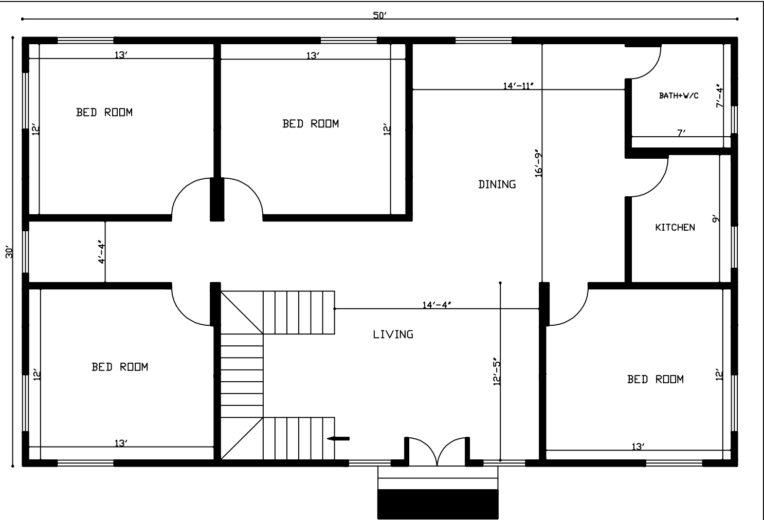
30'X50' 1500 Sq. Ft. House Plan
