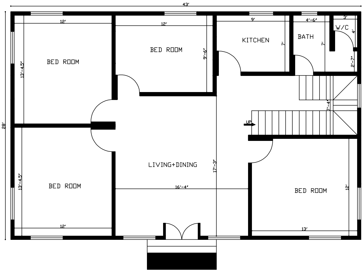
28'x43' 1200 Sq. Ft. House Plan
