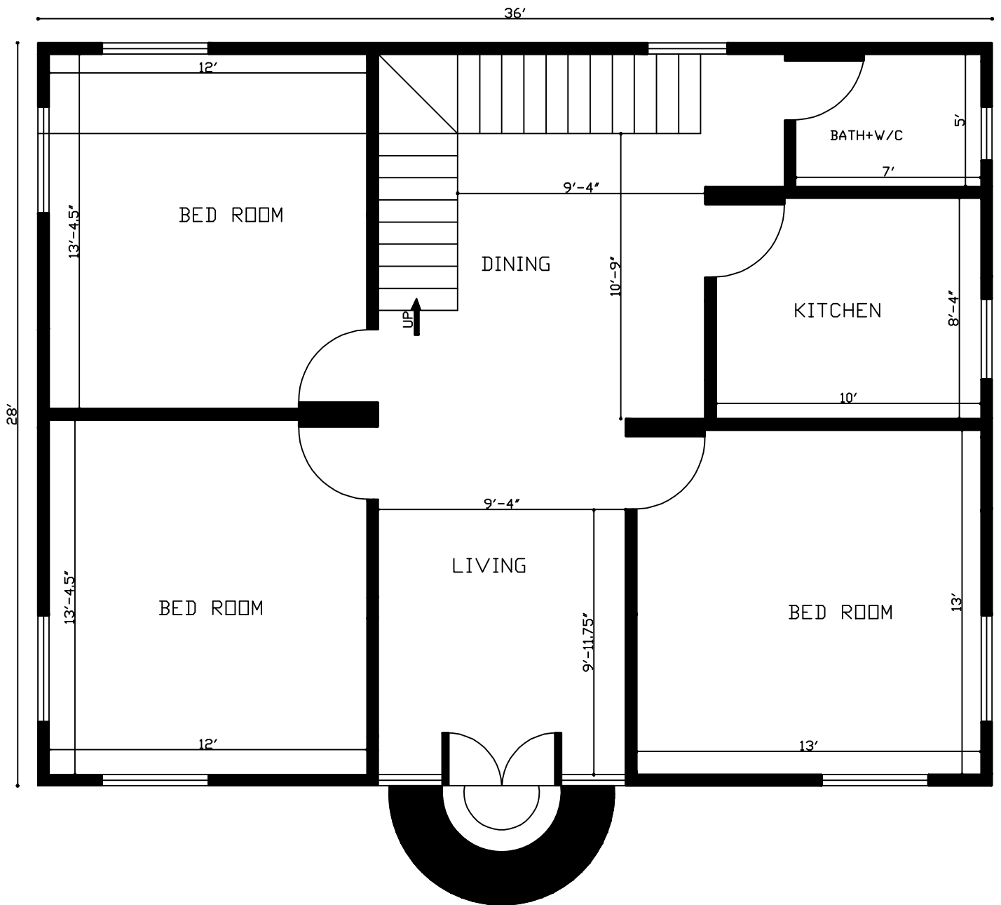
28'x36' 1000 Sq. Ft. House Plan
