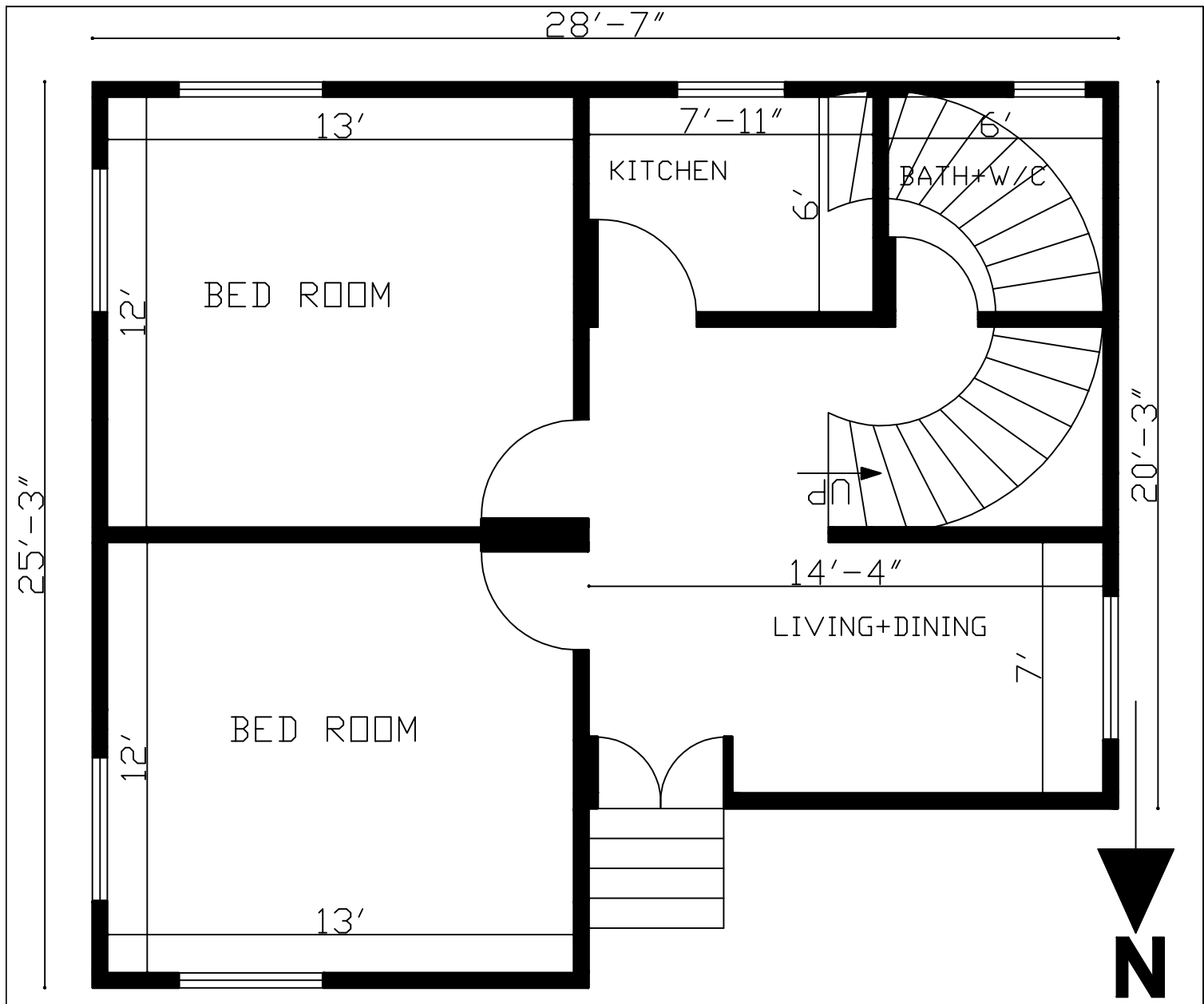
28'x25' 2 BEDROOM HOUSE
