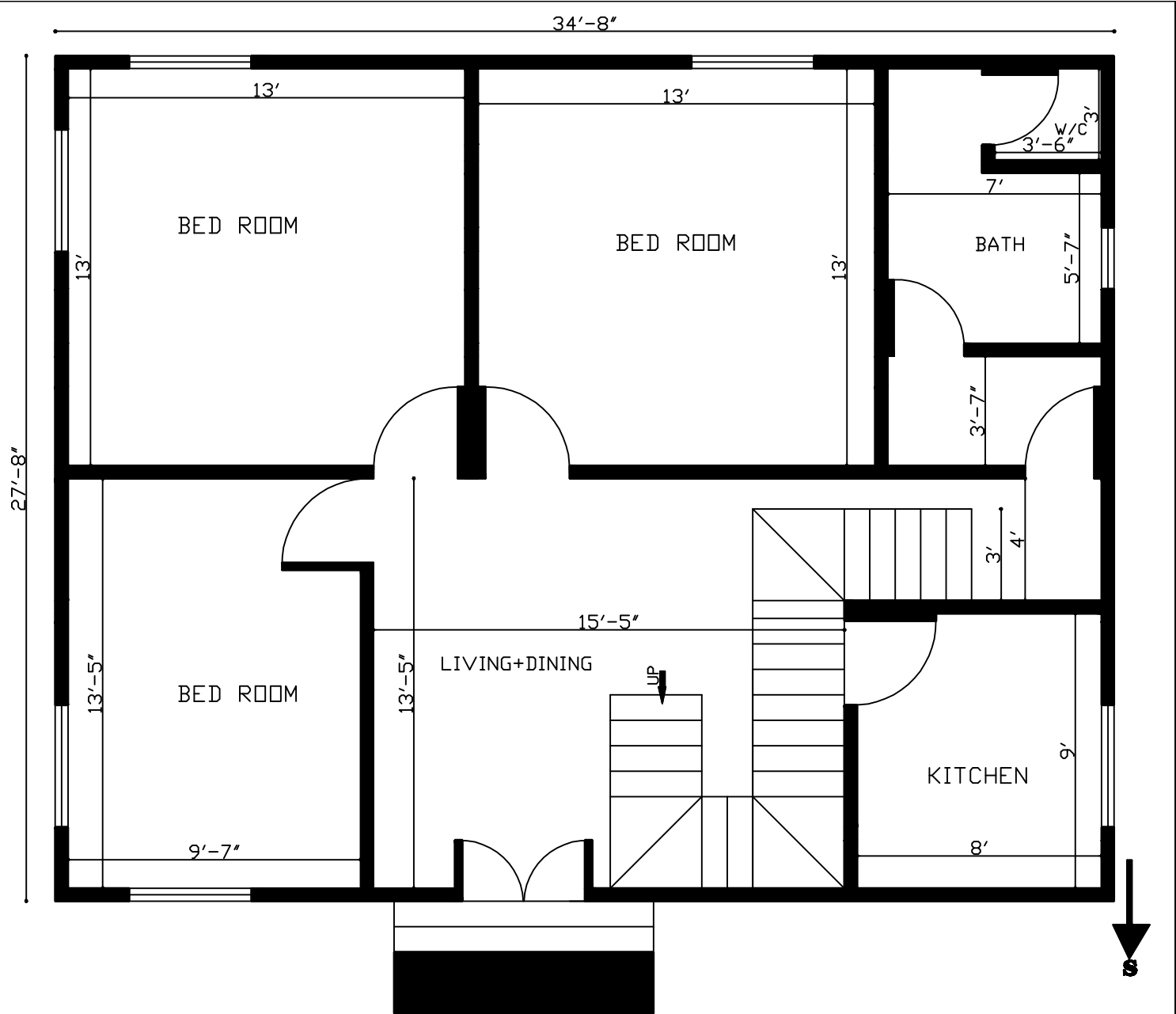
28'X35' 3 Bedroom South Facing House Plan
