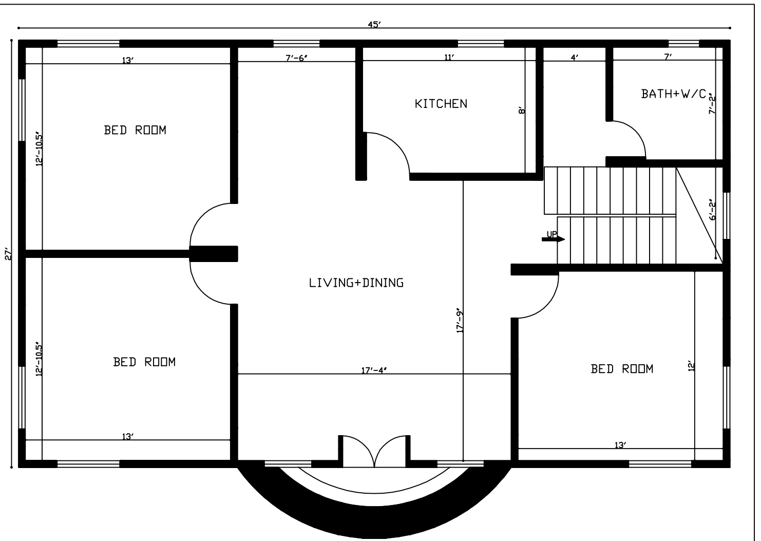
27'x45' 1200 Sq. Ft. House Plan
