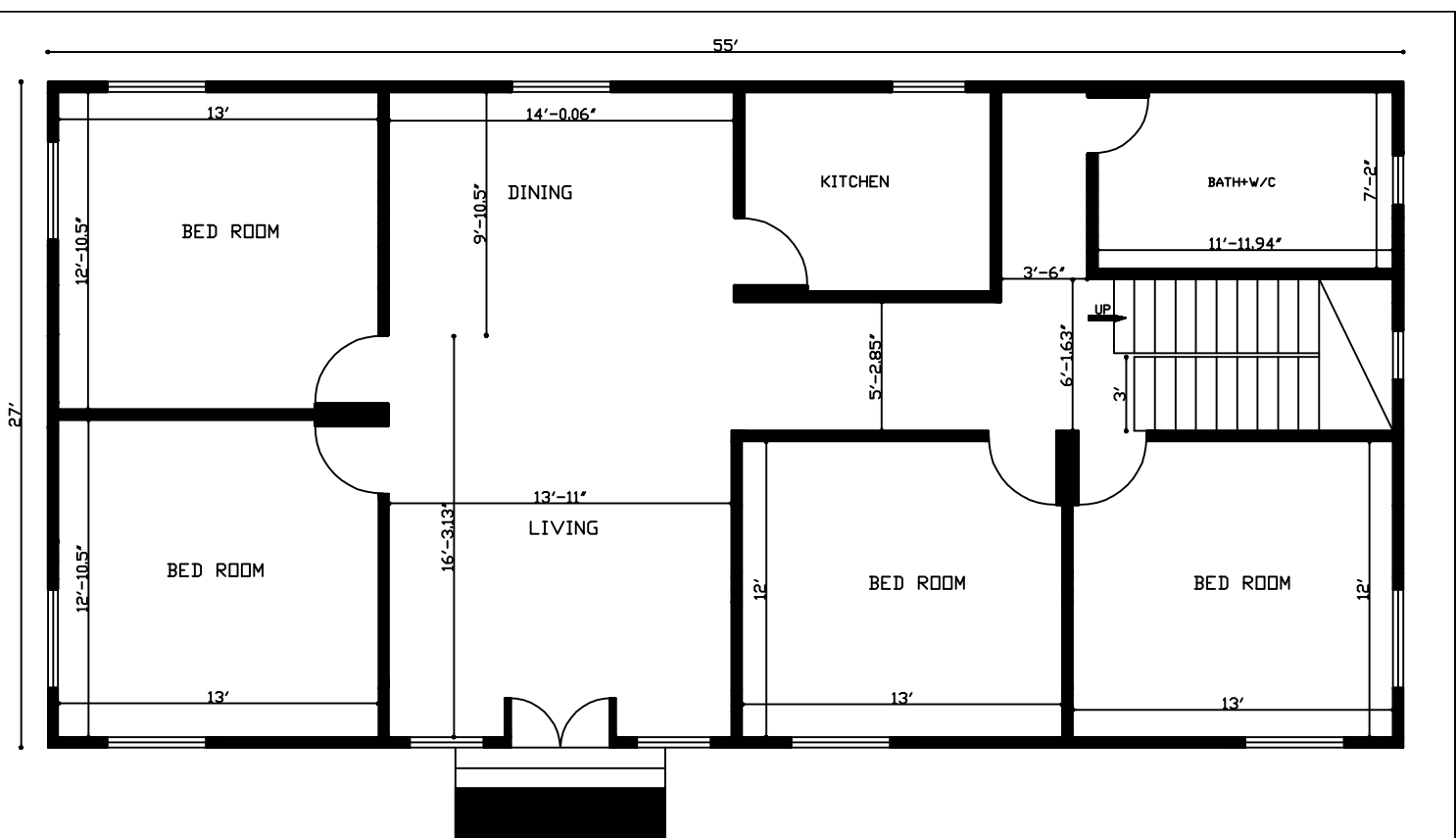
27'X55' 1500 Sq. Ft. House Plan
