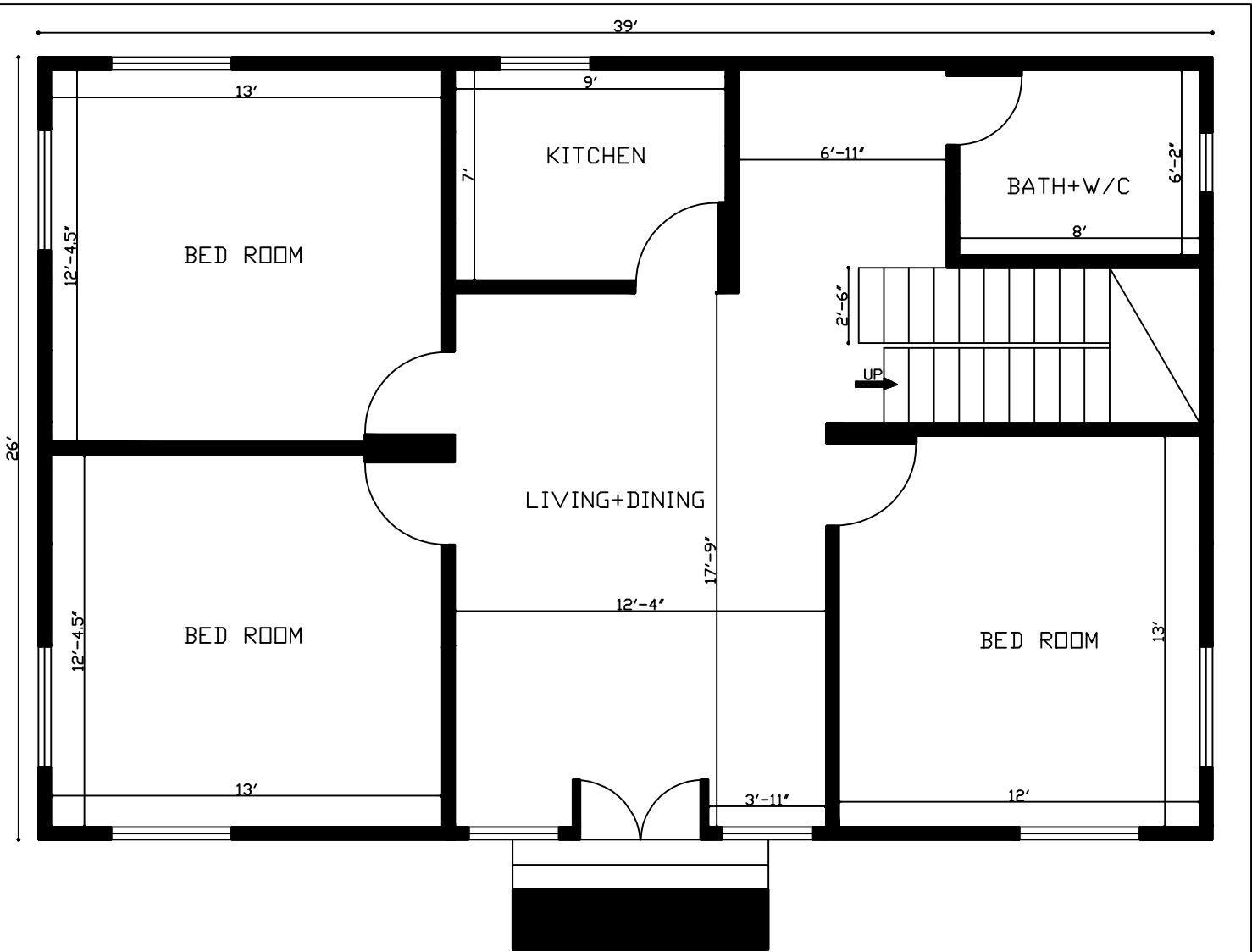
26'x39' 1000 Sq. Ft. House Plan
