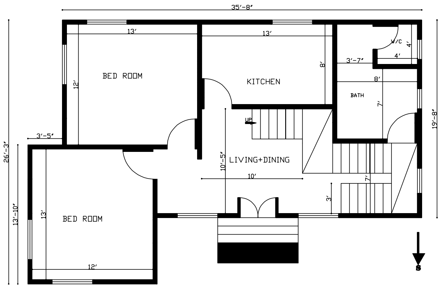
26'X36' 2 Bedroom South Facing House Plan
