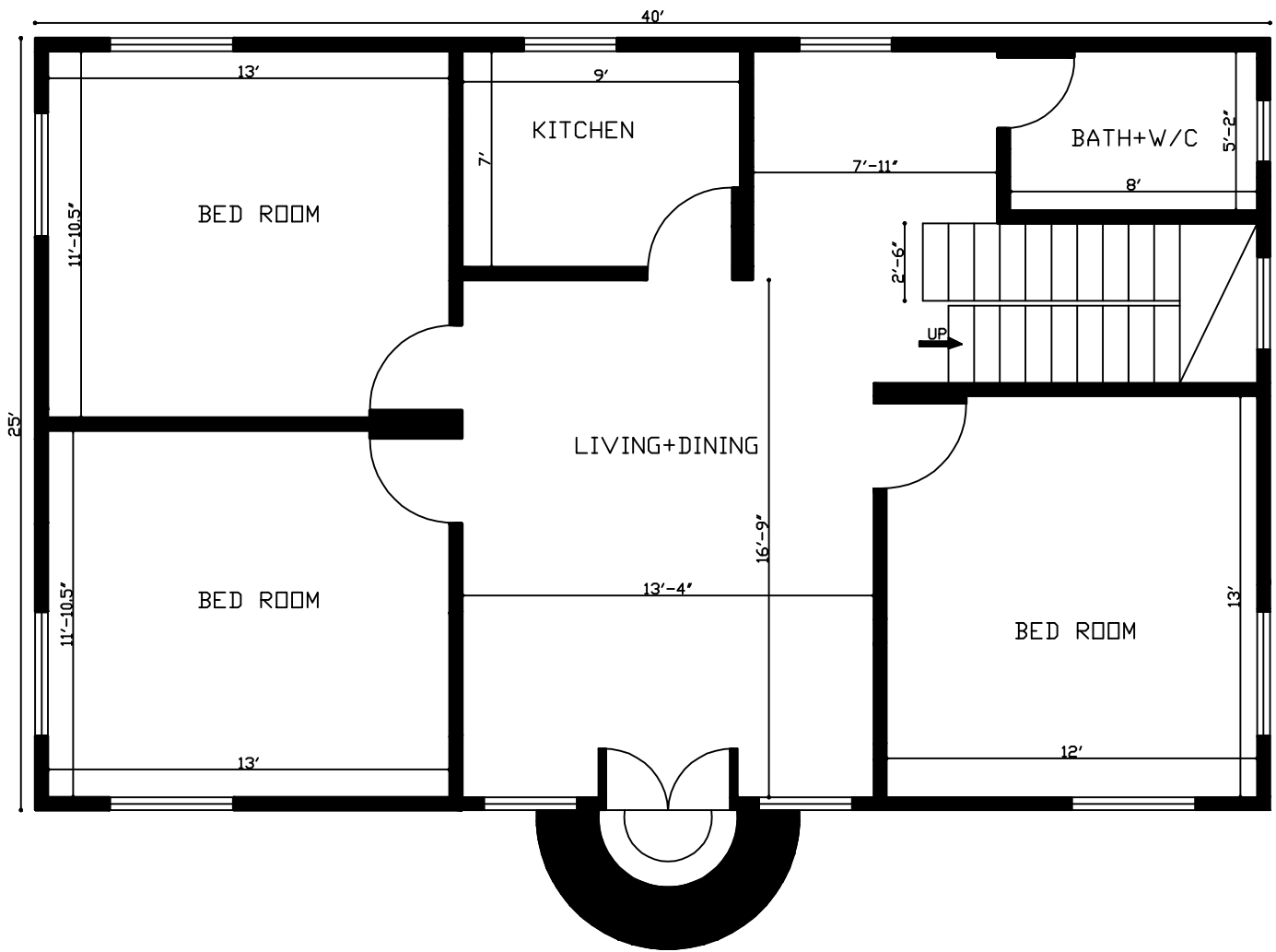
25'x40' 1000 Sq. Ft. House Plan
