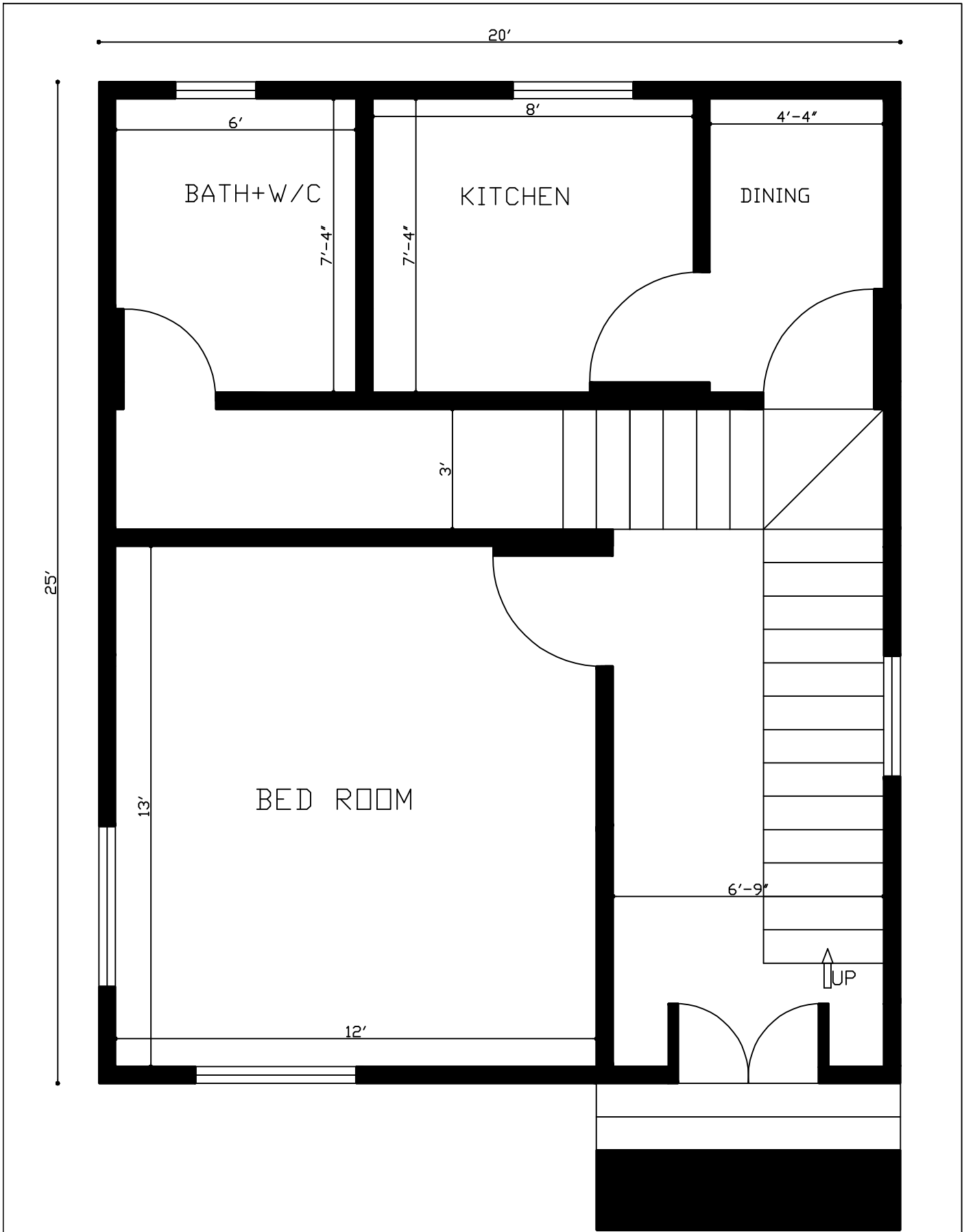
25'x20' 1 Bedroom House Plan
