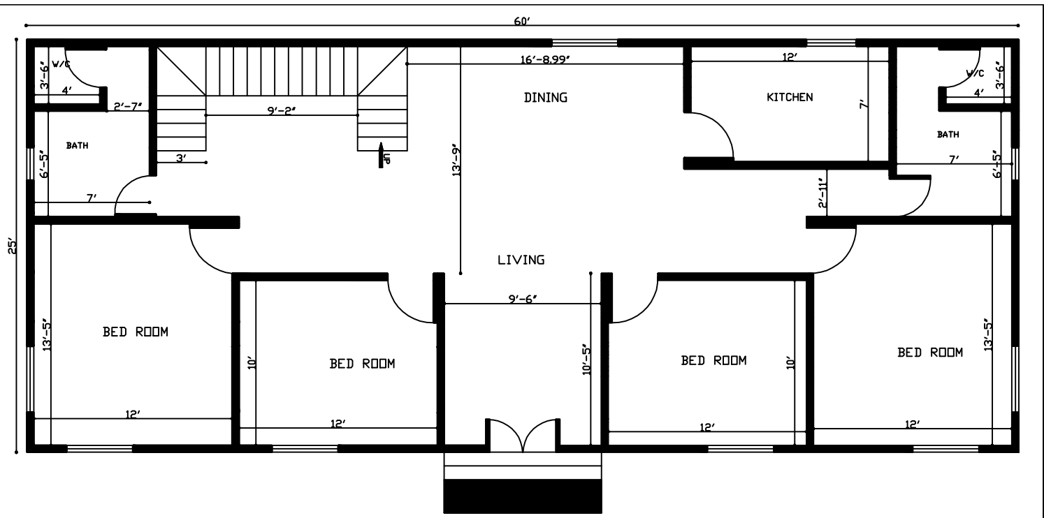
25'X60' 1500 Sq. Ft. House Plan
