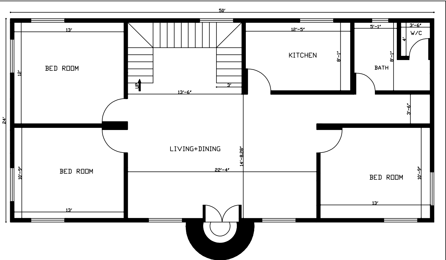
24'x50' 1200 Sq. Ft. House Plan
