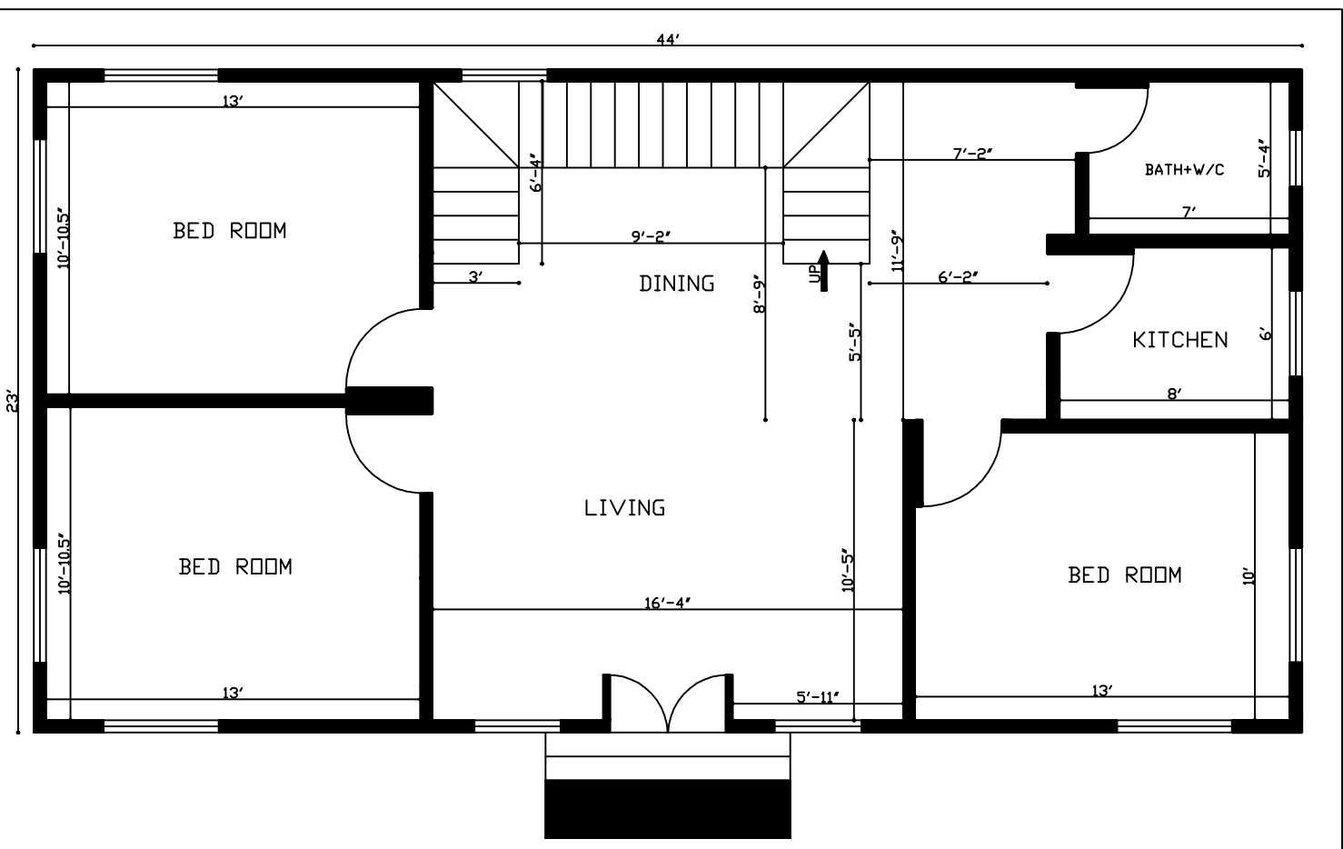
23'x44' 1000 Sq. Ft. House Plan
