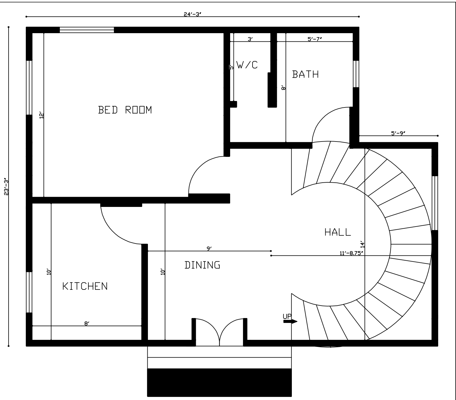
23'x24' 1 Bhk House Plan
