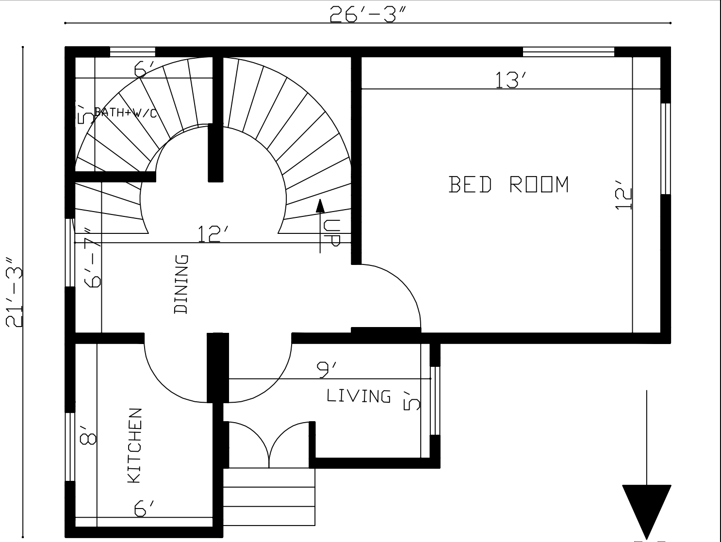
21'x26' 1 BEDROOM HOUSE
