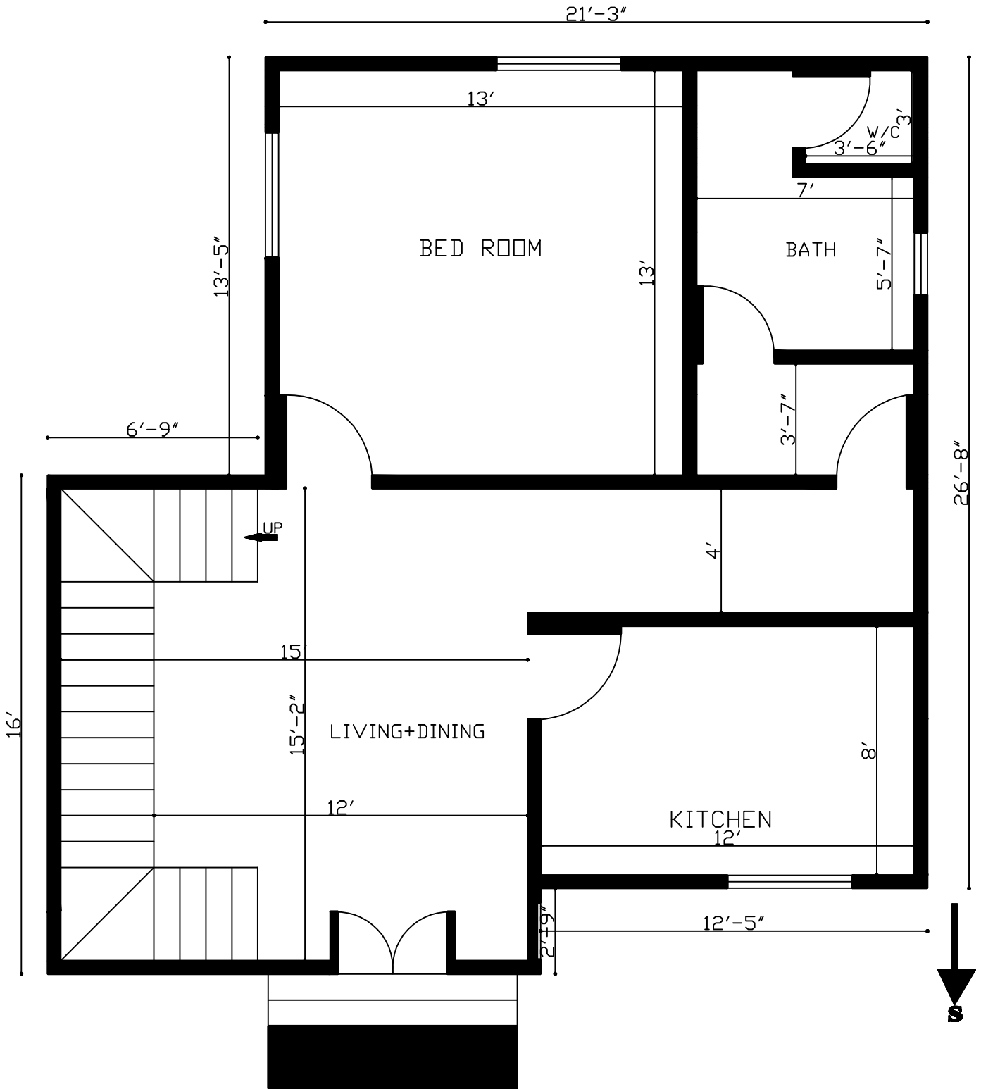
21'X27' 1 Bedroom South Facing House Plan
