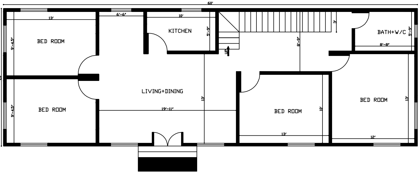
20'x60' 1200 Sq. Ft. House Plan
