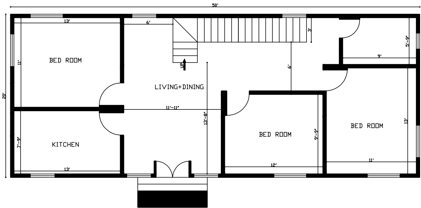
20'x50' 1000 Sq. Ft. House Plan
