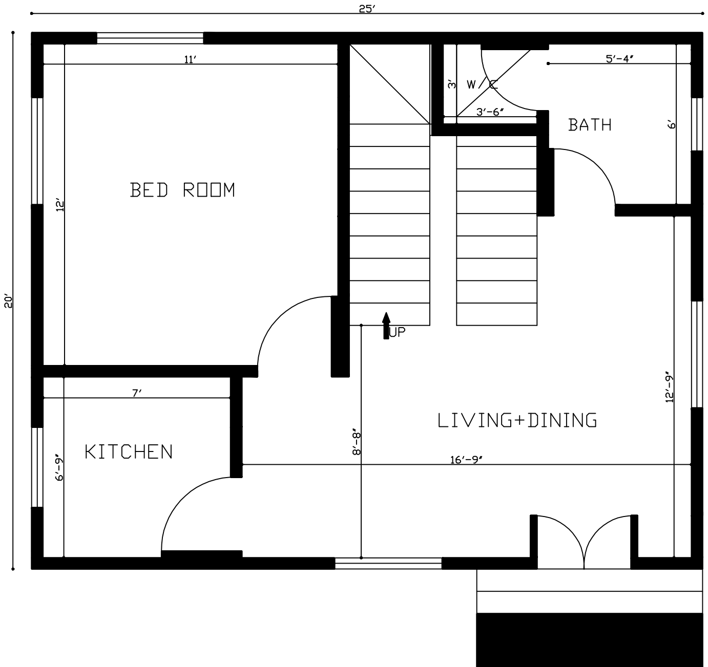
20'x25' 1 Bedroom House Plan
