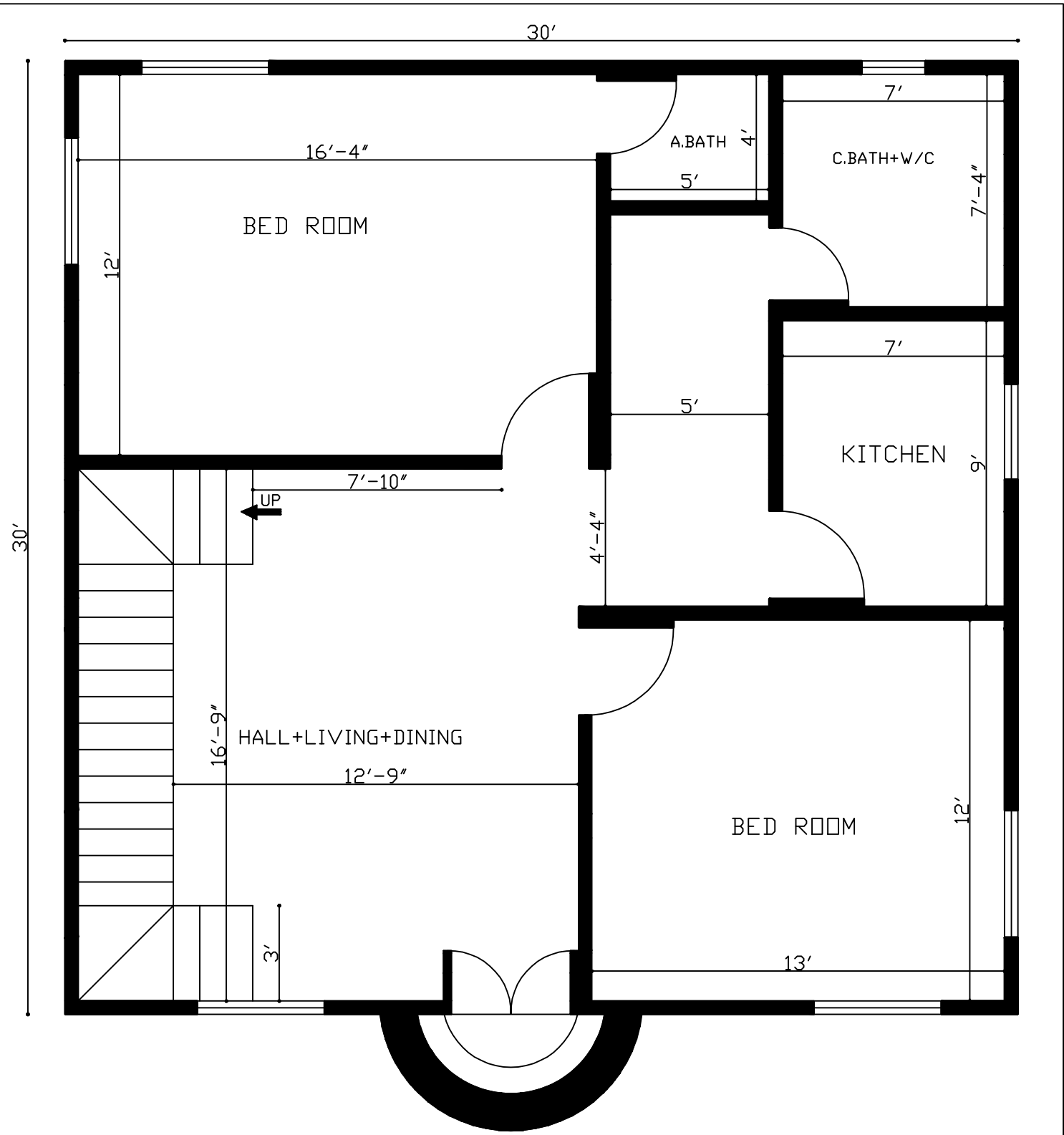
2 Bhk House Plan In 900 Sq. Ft.
