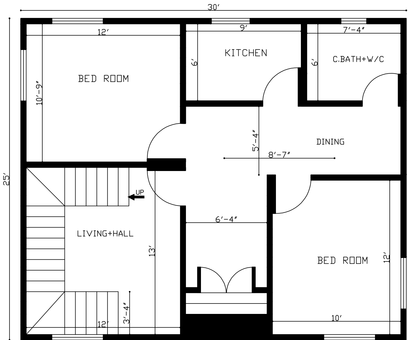
2 Bhk House Plan In 750 Sq. Ft.
