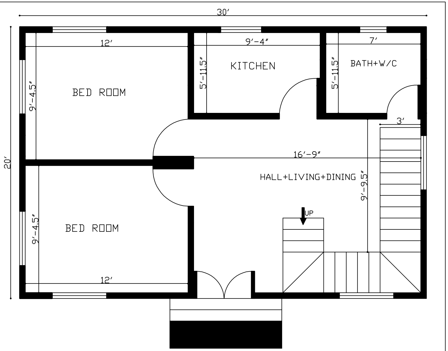
2 Bhk House Plan In 600 Sq. Ft.
