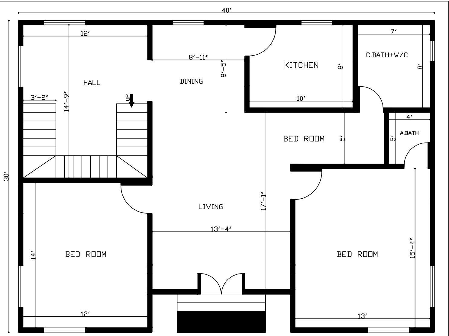
2 Bhk House Plan In 1200 Sq. Ft.
