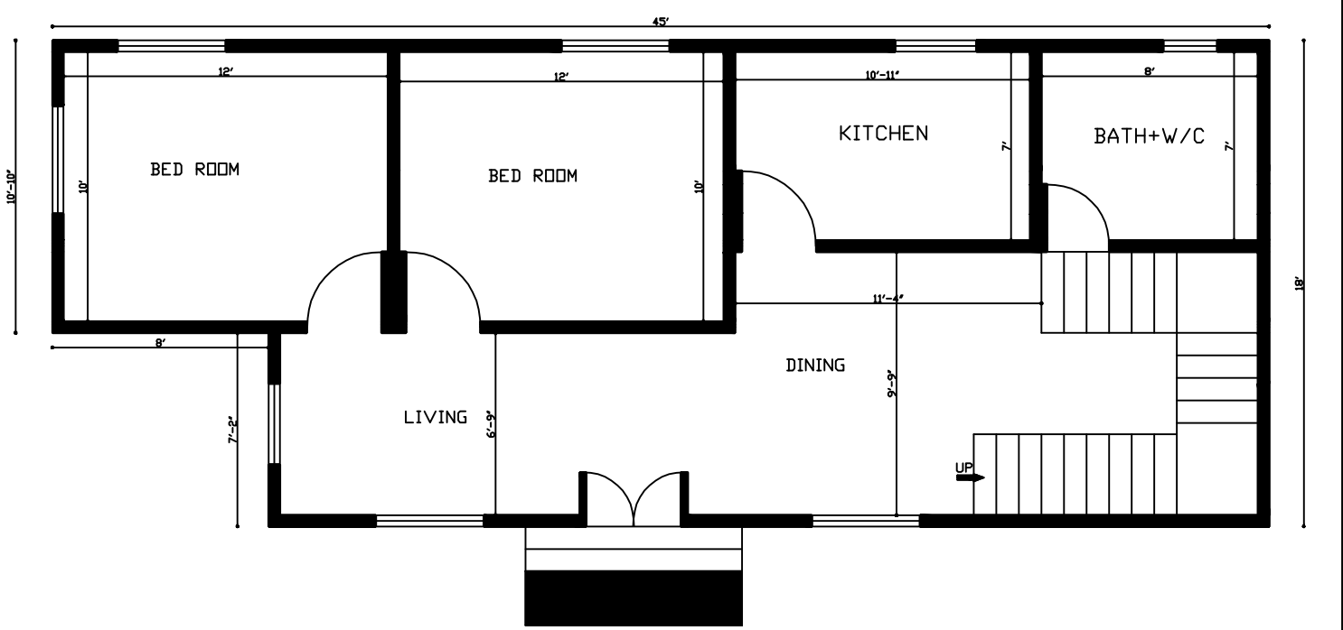
18'x45' 2 Bedroom House Plan
