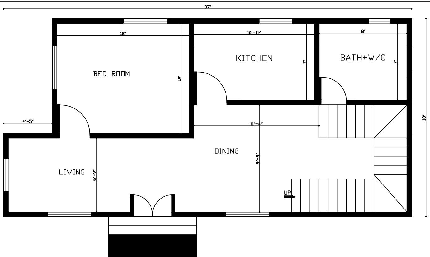
18'x37' 1 Bedroom House Plan
