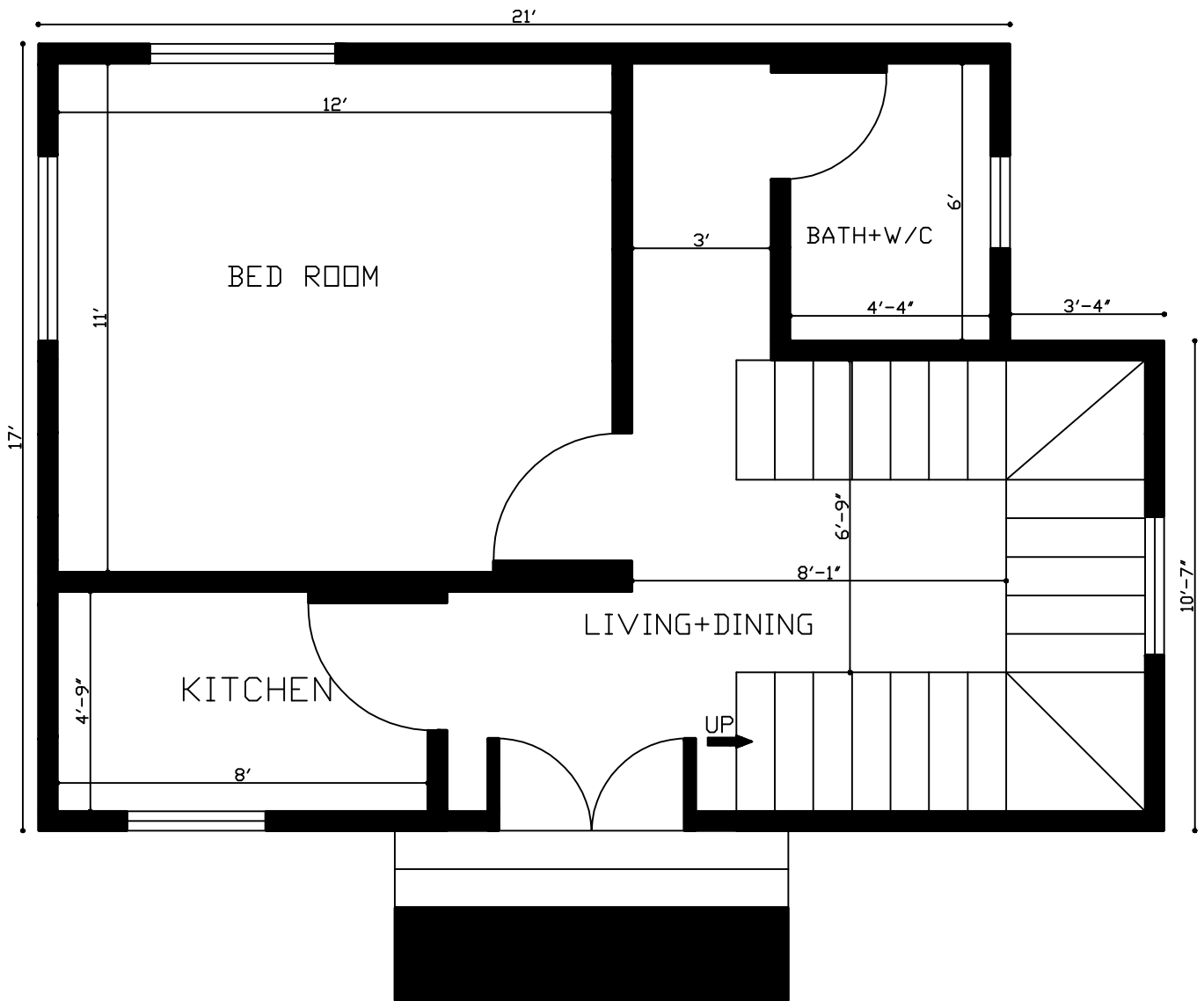
17'x21' 1 Bedroom House Plan
