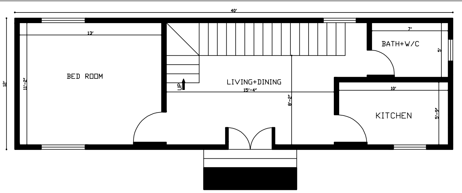
12'x40' 1 Bedroom House Plan
